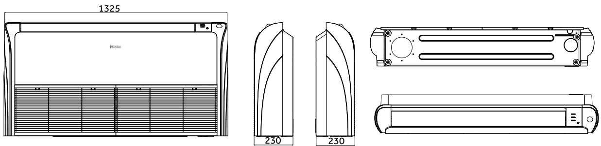
AC71S2SG1FA, AC105S2SH1FA
