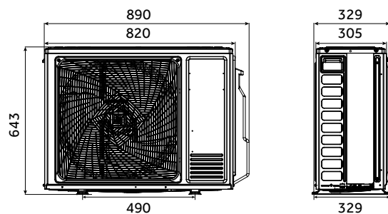
1U50S2SJ3FA
