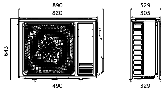
1U50JEC1FRA
