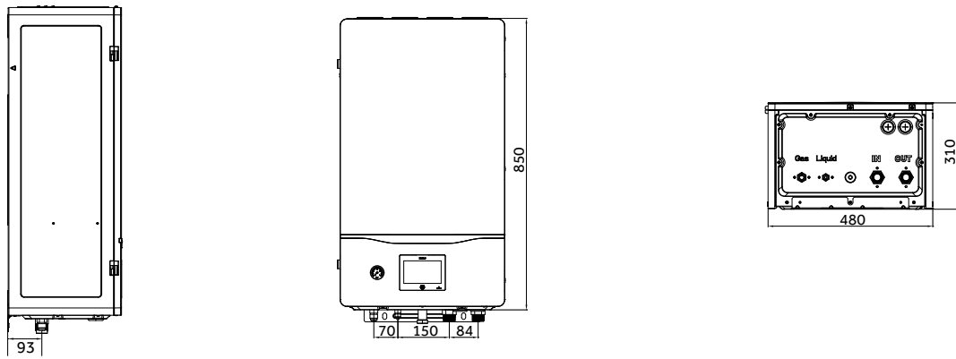
HU062WAMNA, HU102WAMNA
