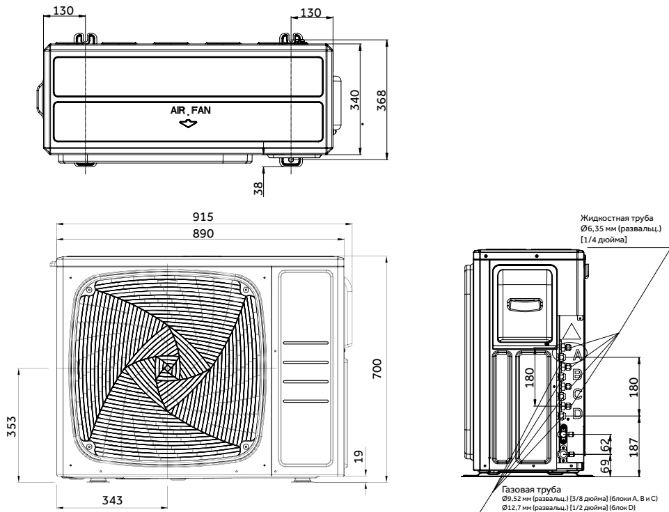
4U75S2SR5FA, 4U85S2SR5FA
