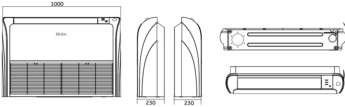
AC35S2SG1FA, AC50S2SG1FA
