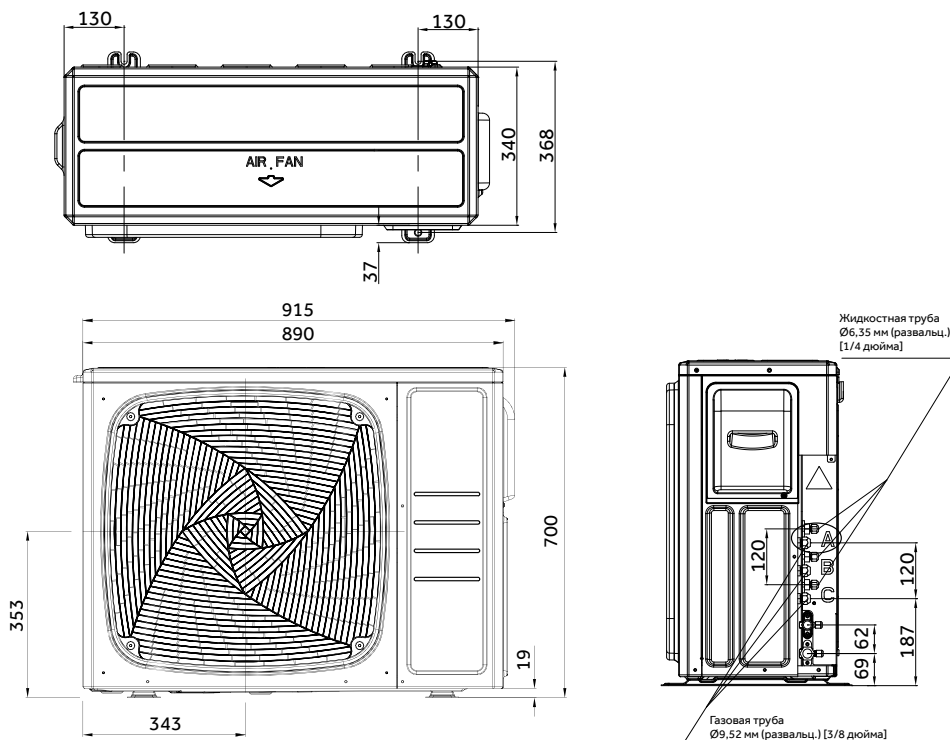
3U55S2SR5FA, 3U70S2SR5FA
