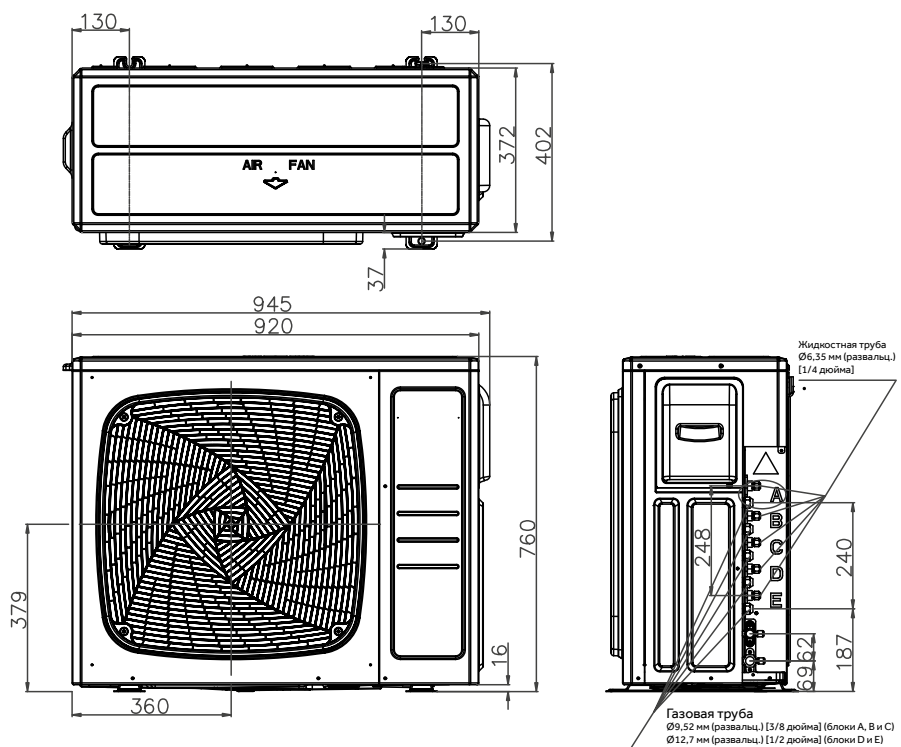
5U90S2SS5FA, 5U105S2SS5FA
