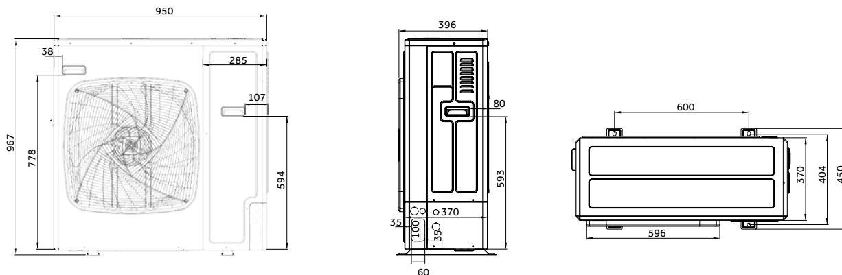
1UH071N1ERG, 1UH105N1ERG
